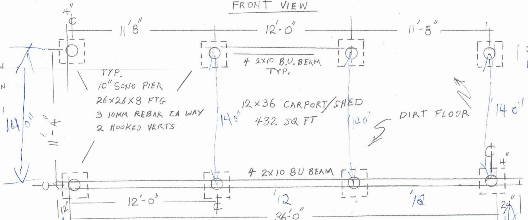
PLAN VIEW
