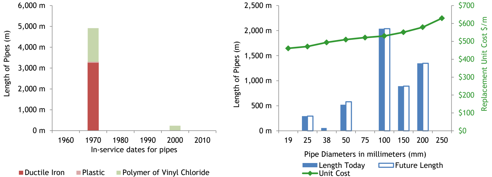
Figure 2: Ymir Pipe Distribution Network (Length, Material, Diameter)
