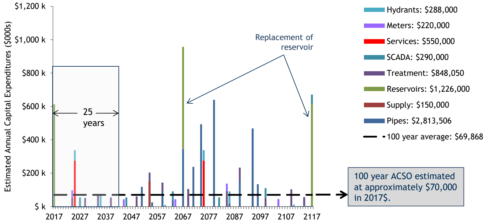
Figure 6: Ymir 100 Year Asset Replacement Schedule
