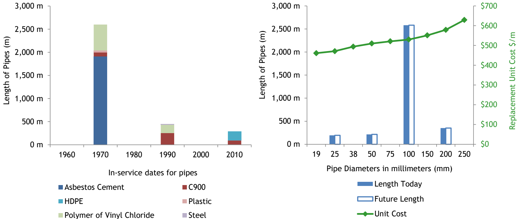
Figure 2: Duhamel Pipe Distribution Network (Length, Material, Diameter)
